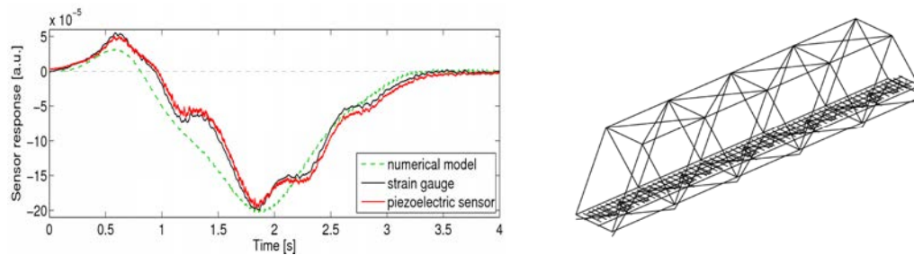
Figure 9. Comparison of numerical and experimental results at selected point.
