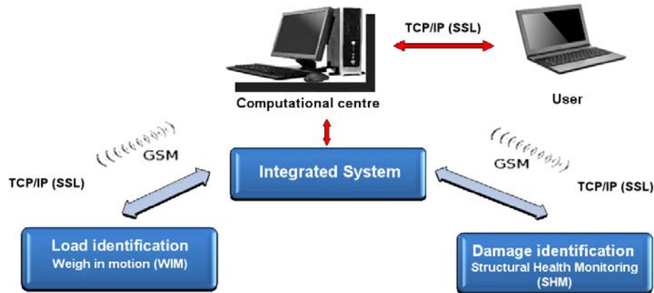
Figure 2. Scheme of the integrated system.
