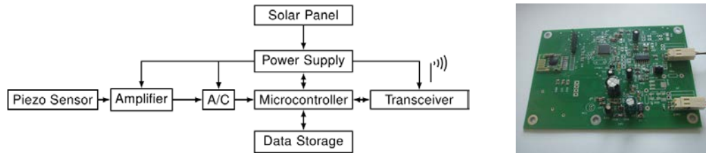
Figure 8. Wireless sensor: block diagram and PCB implementation.
