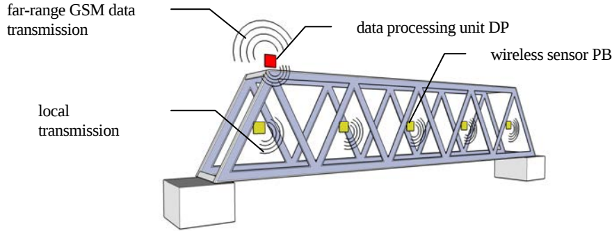
Figure 6. SHM piezoelectric sensor.
