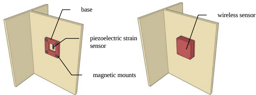
Figure 7. Mounting of wireless SHM sensor.
