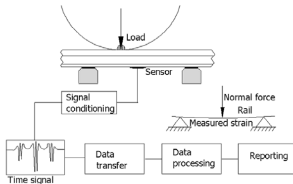
Figure 3. WIM subsystem.
