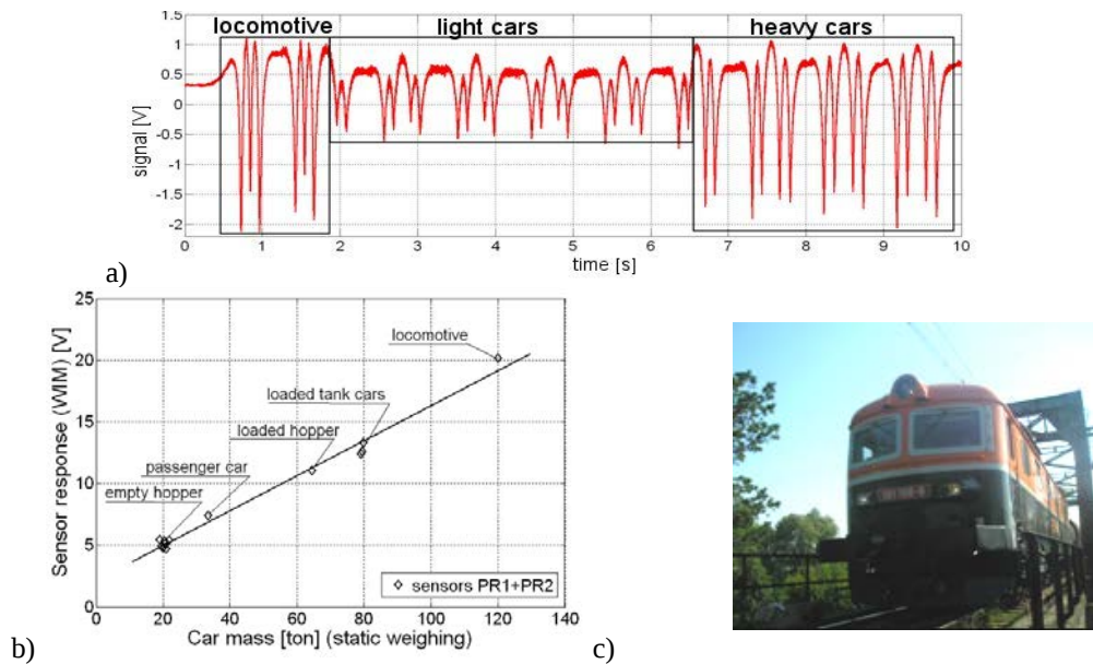
Figure 5. Results of mass identification from the WIM subsystem.
